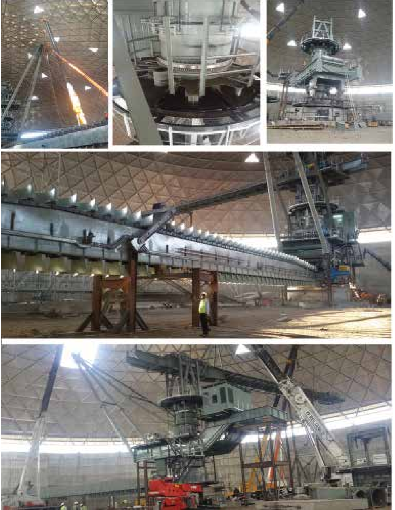
Circular Stacker Reclaimer for Coke Storage Erected at Reliance Refinery, Gujarat, India
